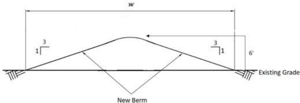
Figure 2: Berm Diagram
